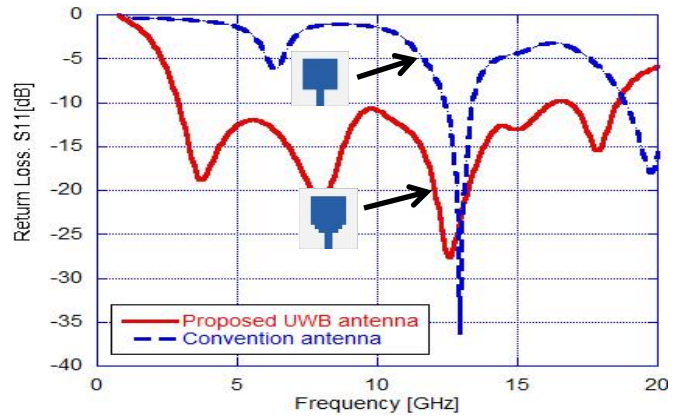
Figure 2: The proposed antenna versus conventional one.
